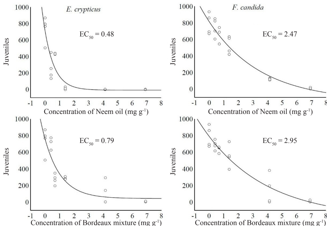
Figure 2. Exponential regression and effective concentration values (EC 50 ) for juveniles of E. crypticus and F. candida submitted to increasing doses of Neem oil and Bordeaux mixture. Values of the confidence interval of the estimates (CL95%): Neem oil in E. crypticus (0.25-0.70) and F. candida (0.88 - 4.06); Bordeaux mixture in E. crypticus (0.36 - 1.21) and F. candida (0.32 - 5.58).
